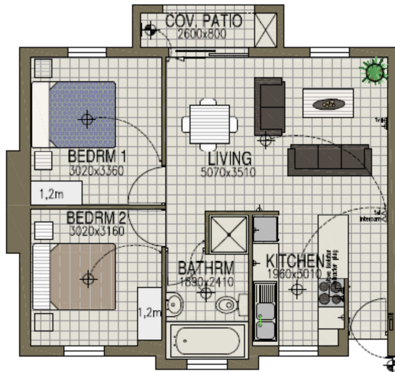
UNIT TYPE 1 ( 65 Sq/M ) SCALE 1:50
